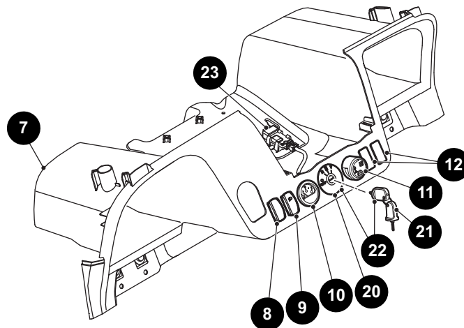
with Horn/Lights/SOC/USB
