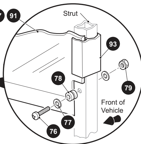
FULL WINDSHIELD
