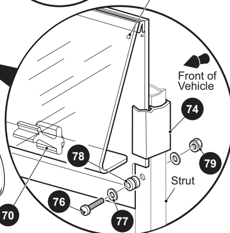
SPLIT WINDSHIELD
